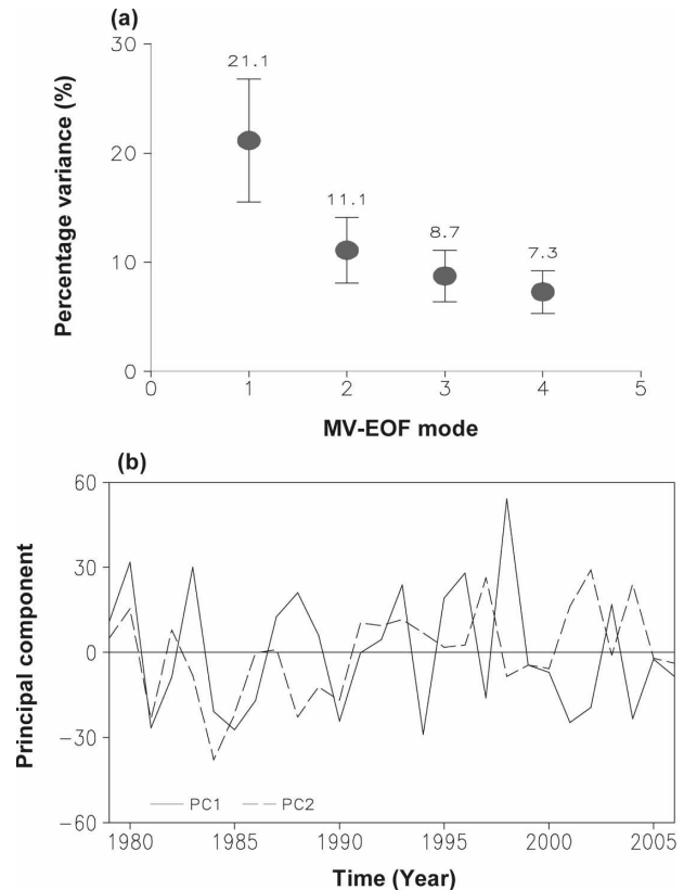
FIG. 1. (a) Fractional variance (%) explained by the first four MV-EOF modes and the associated unit standard deviation of the sampling errors. (b) PCs of the first and second MV-EOF modes.
